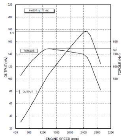
Engine performance curve 6M60-9AT1
